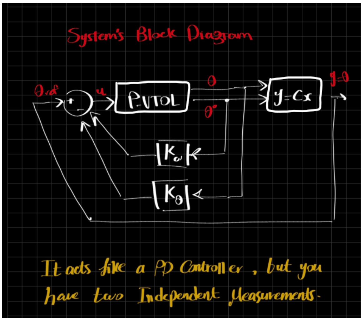
Figure 6: System's Block Diagram
